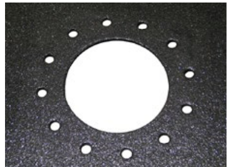
Figure 5. An ASME Class 150 Flat Face Flange Pattern is Shown on this Cold Water Basin Panel
