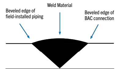
Figure 1. Weld Details
