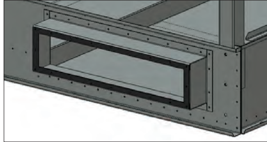
Figure 12. Flume Box Butyl Sealer Tape Application
