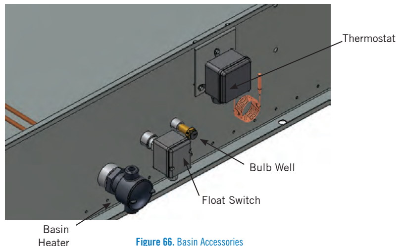
Figure 66. Basin Accessories
