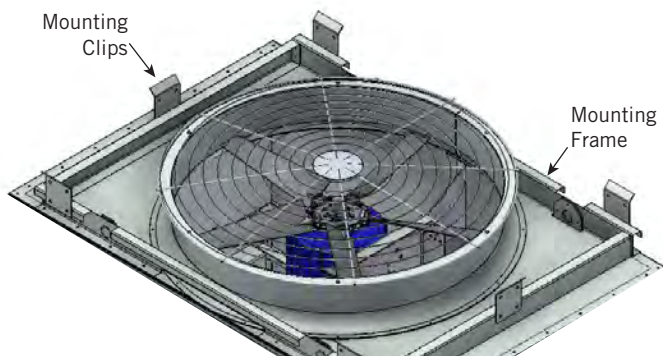
Figure 25a. Position of Discharge Sound Attenuation Clips
