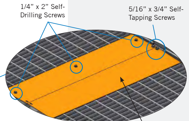
Detail C
