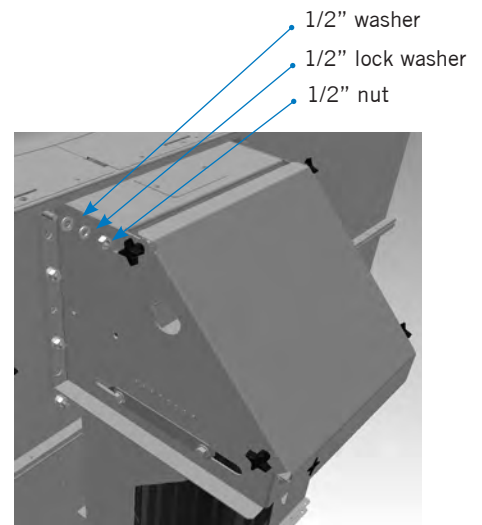
Figure 18. External Motor Mount Assembly Pattern
