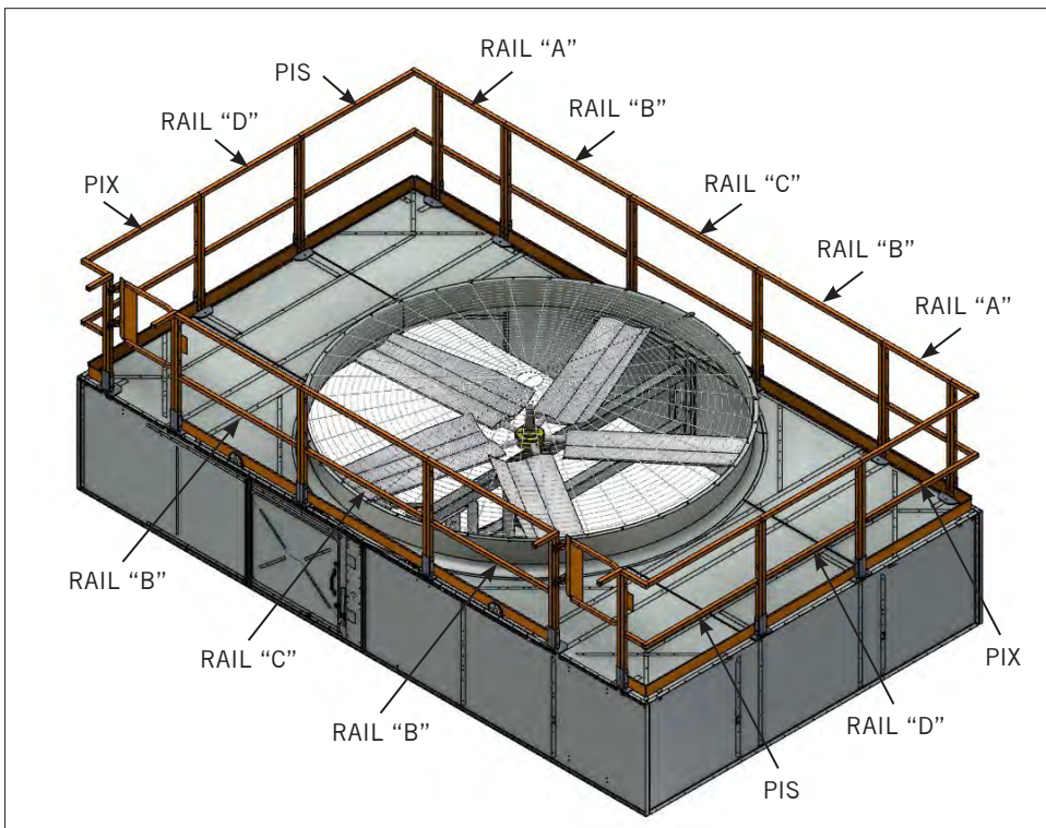
Figure 49. Top Perimeter Guardrails - PFi/PCC-1218, 1220
