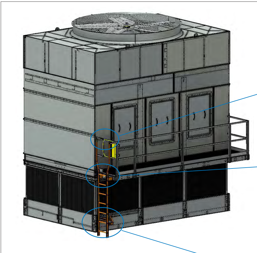
Figure 47. Fill Access Platform End Ladder – All units
