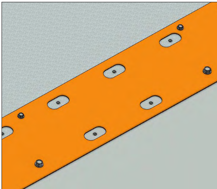
Figure 59. Top Perimeter Guardrail Gap Plate Attachment
