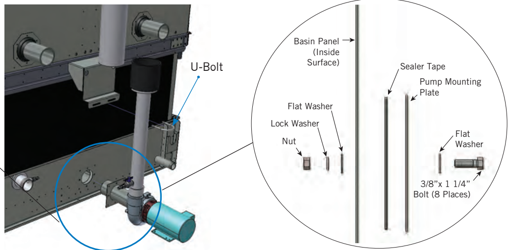
Detail A
