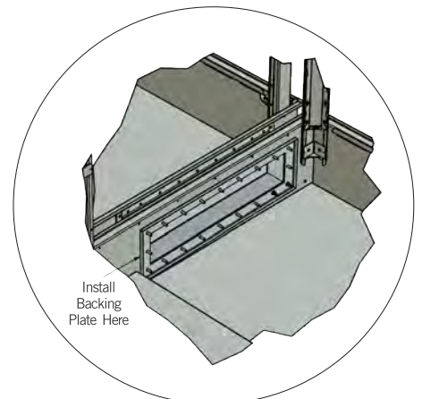
Figure 14. Backing Plate Installation
