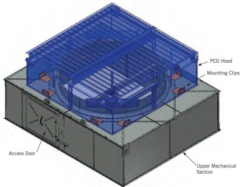
Figure 24. PCD Hood Bracket Mounted Assembly
