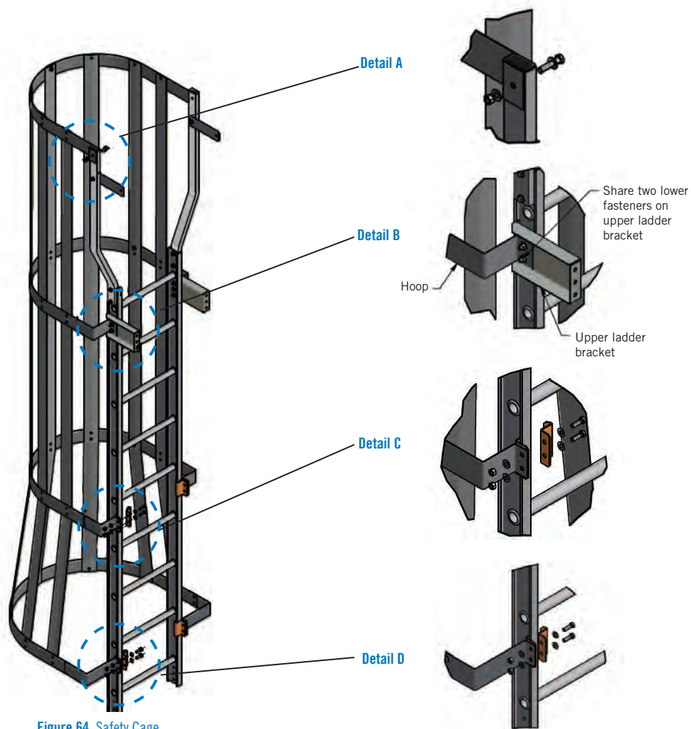
Figure 64. Safety Cage
