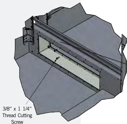
Figure 13. Thread Cutting Screw Pattern for Flume Box
