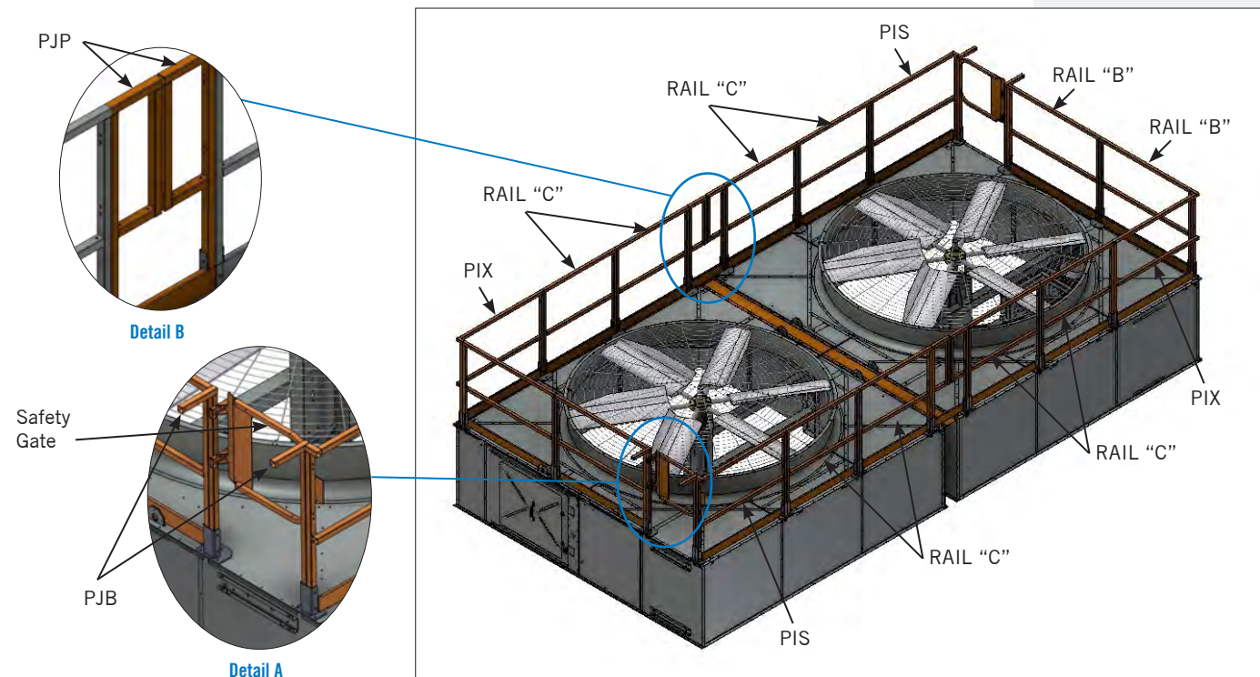
Figure 50. Top Perimeter Guardrails - PFi/PCC-2412
