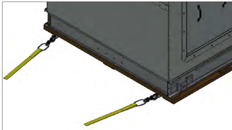
Figure 9. Removing Unit from Container Using Pulling Lugs
