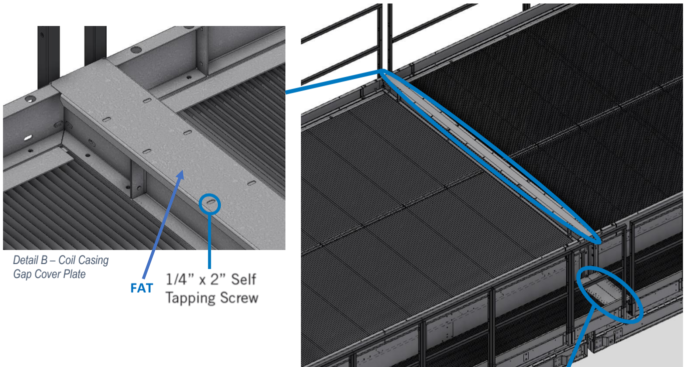
Figure 20. Gap Cover Plate Location & Installation (model details hidden for clarity)
