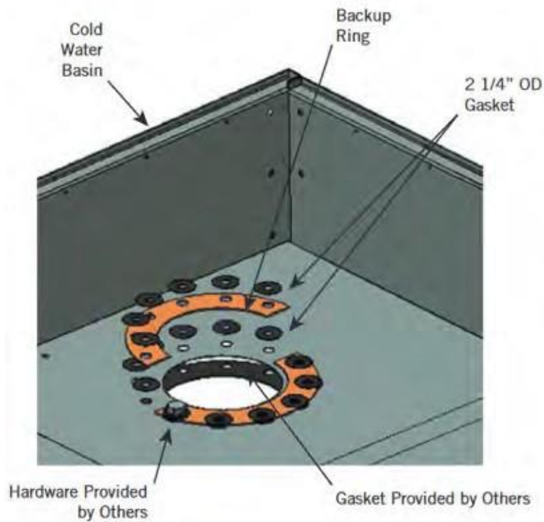
Figure 6. Bottom Water Outlet
