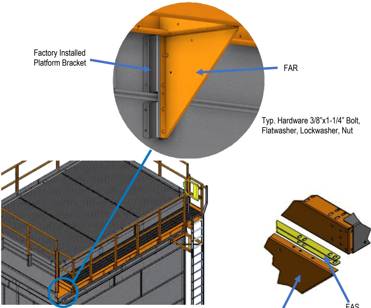
Figure 7. Typical Offset Platform Installation
