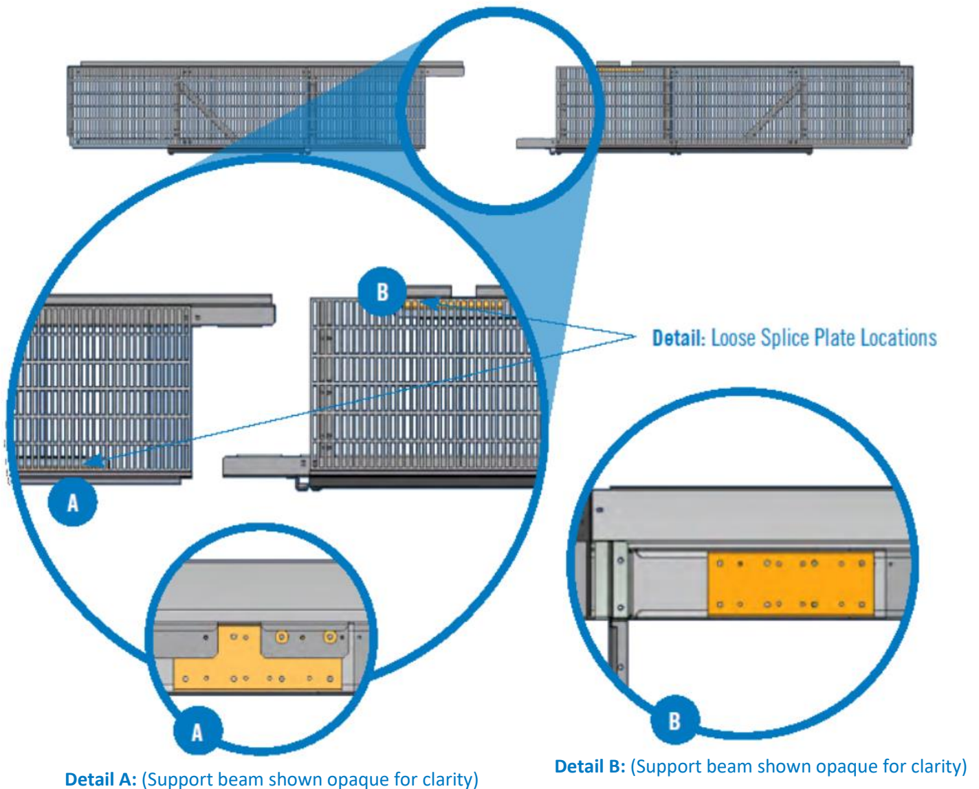
Figure 13. Two Platform Sections
