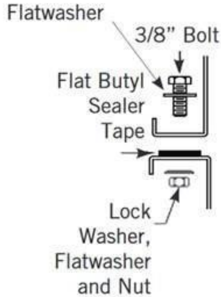
Figure 5. Fastening of Upper and Lower Sections
