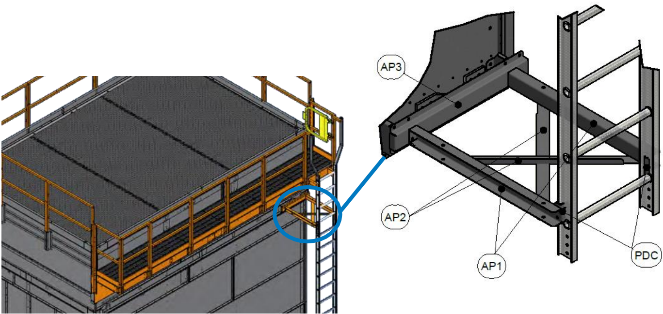
Figure 9. Typ. Ladder & Bracket Installation
