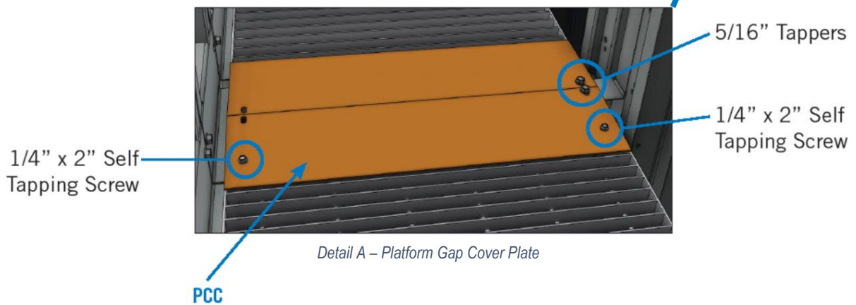
Figure 20. Gap Cover Plate Location & Installation (model details hidden for clarity)
