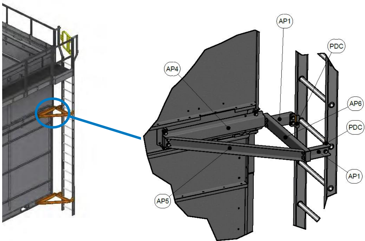
Figure 10. Typ. End Ladder & Bracket Installation
