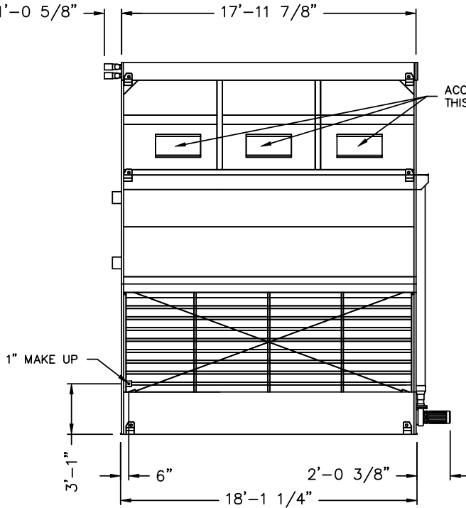
SIDE ELEVATION
