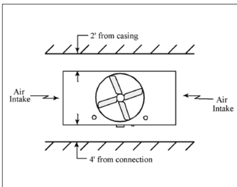
Figure 1. Plan view of Recommended Unit Servicing and Maintenance Spacing for Dual Air Inlet Unit (FXV-288 & 364 Closed Circuit Cooling Towers, CXV-T Evaporative Condensers)
