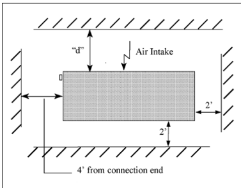
Figure 2. Plan View of Recommended Unit Servicing and Maintenance Spacing for Single Air Inlet Unit (FXV Closed Circuit Cooling Towers, CXVB Evaporative Condensers)
