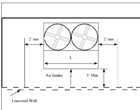
Figure 7. Plan View of Single Air Inlet Unit in Enclosure with Louvered Walls
