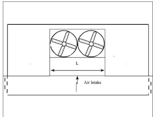
Figure 9. Plan View of Single Air Inlet Unit with Alternate Louver Arrangement
