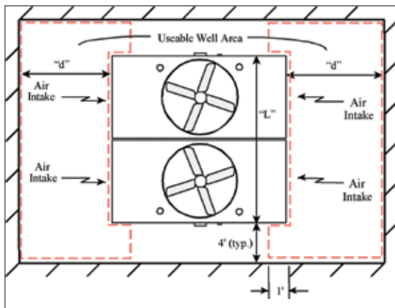
Figure 4. Plan View of Dual Air Inlet Unit in a Well Enclosure
