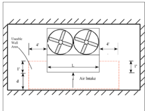
Figure 5. Plan view of Single Air Inlet Unit in a Well Enclosure
